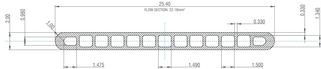
MULTI-PORT EXTRUSION TUBE 25.4/2.0-13-MP SECTIONAL VIEW 10:1
