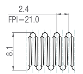
AIRSIDE FINS L25.4-8.1/0.08-21.0 LOUVERED-TYPE 5:1
